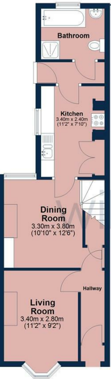
Ground Floor Approx. 41.3 sq. metres (444.9 sq. feet)
